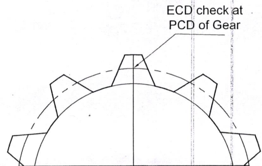
Gear Profile
